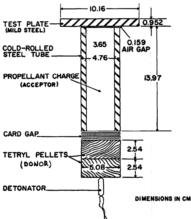
Fig 2 LSGT Assembly
